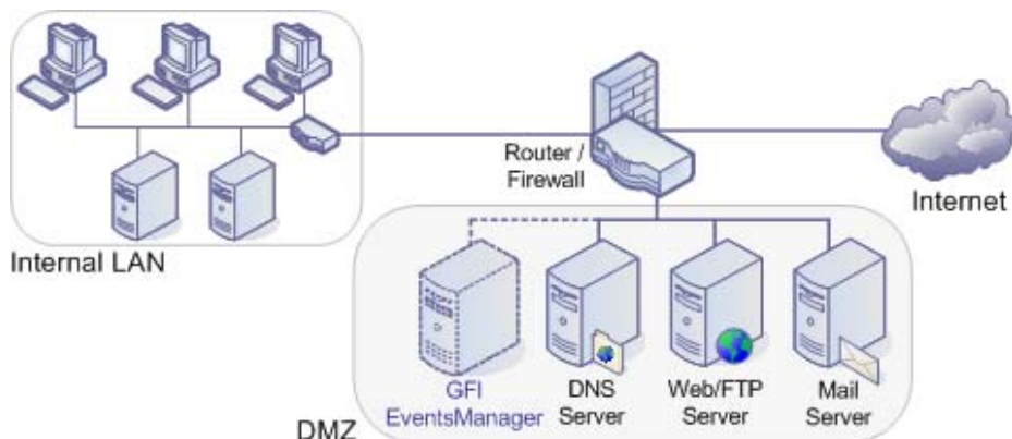
Figure 5 - The DMZ sits between the internal LAN and the Internet
