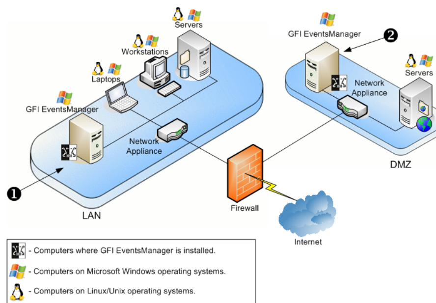
Figure 3 – GFI EventsManager deployment scenario
